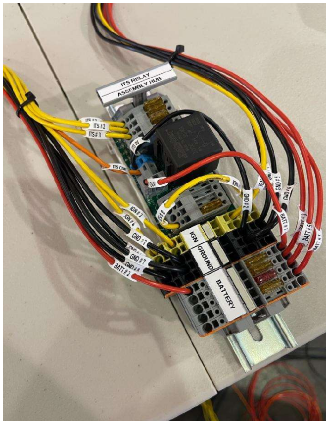
Organized & Labeled Power Wires for various ITS Equipment
